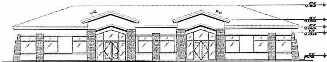
EAST ELEVATION
