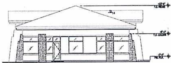
NORTH ELEVATION
